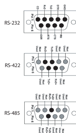
Serial Pin Assignments
